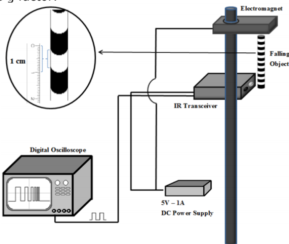
Invention apparatus.
